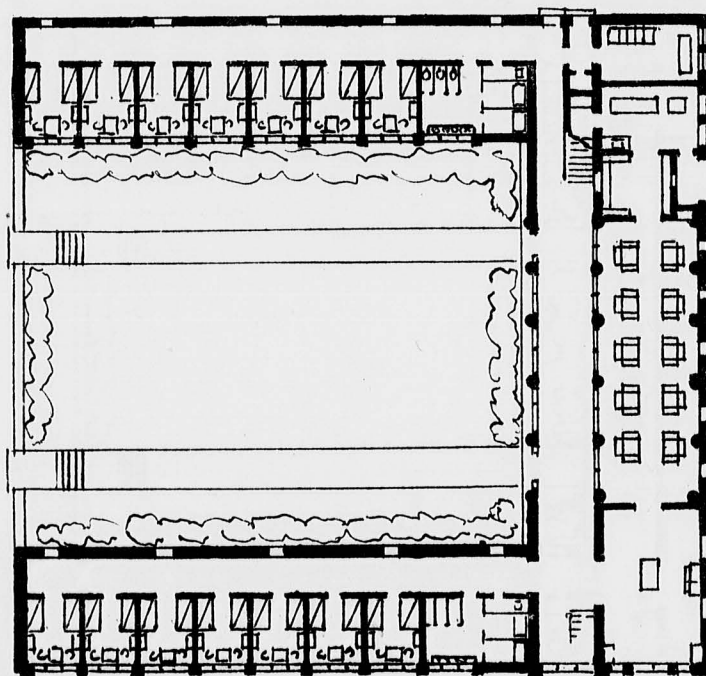
TYPICAL UNIT PLAN.
